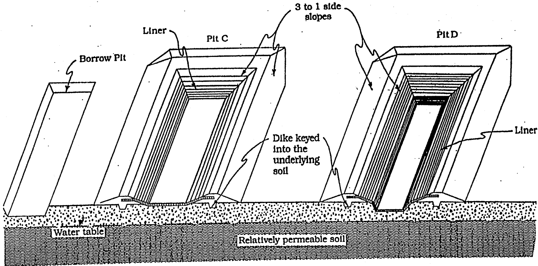
Figure 6 Above-ground pits (lined)
